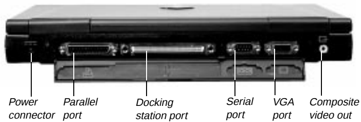
Back ports panel
