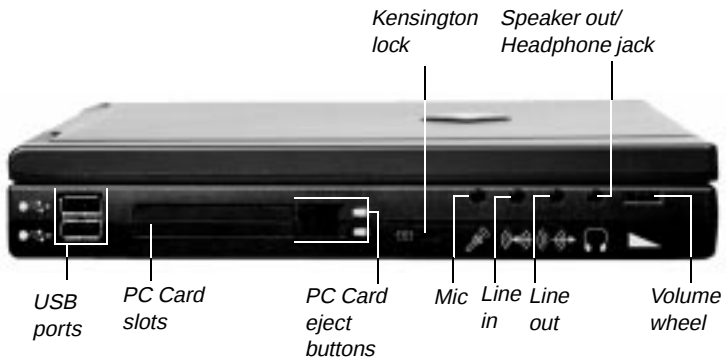
Left side ports and PC Card slots
